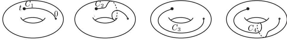
FIGURE 1. Four cuts on \hat{T}
